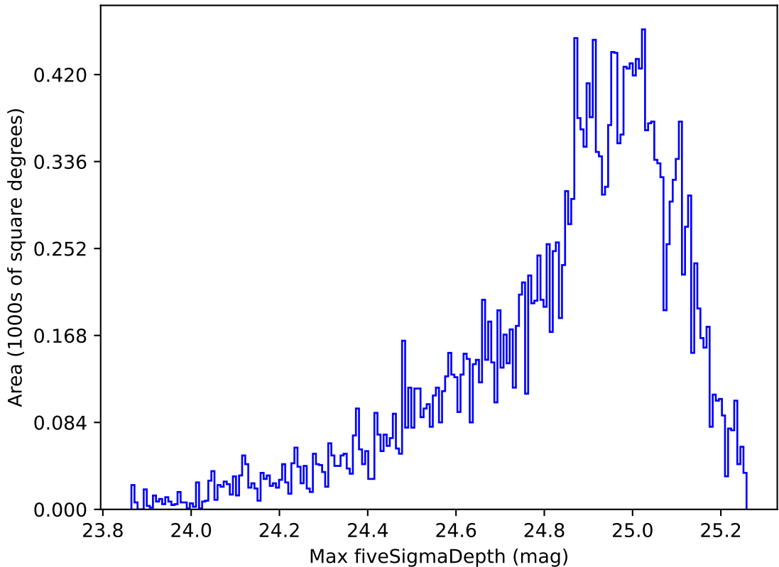
weather_cloudso10v3.4_10yrs Yr 1 all bands: Max fiveSigmaDepth
