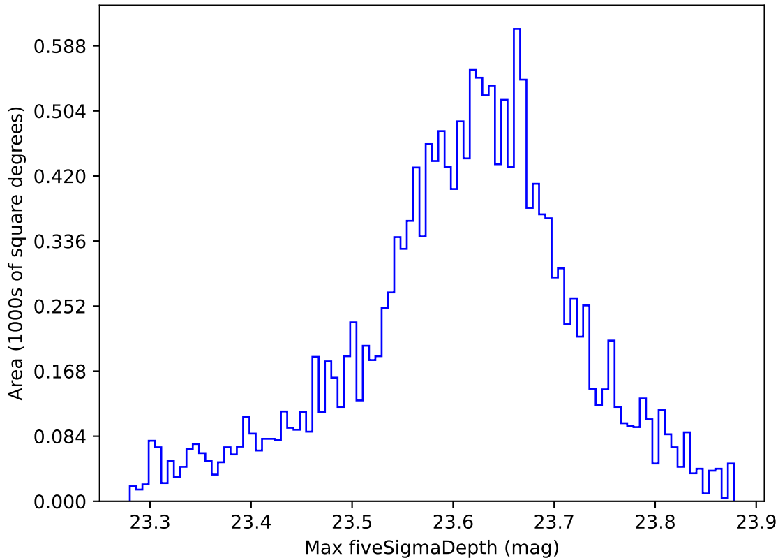
weather_cloudso10v3.4_10yrs WFD z band: Max fiveSigmaDepth
