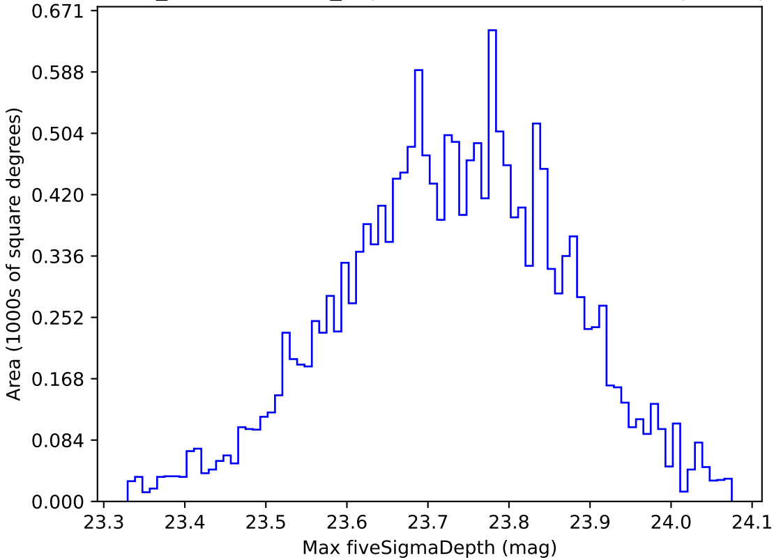
weather_cloudso10v3.4_10yrs WFD u band: Max fiveSigmaDepth
