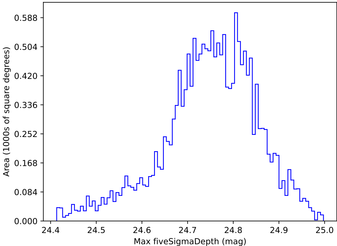
weather_cloudso10v3.4_10yrs WFD r band: Max fiveSigmaDepth
