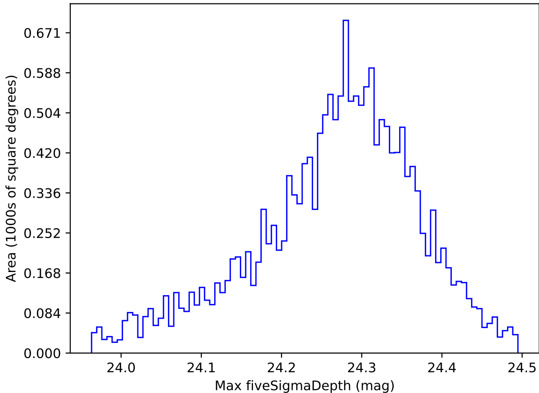
weather_cloudso10v3.4_10yrs WFD i band: Max fiveSigmaDepth
