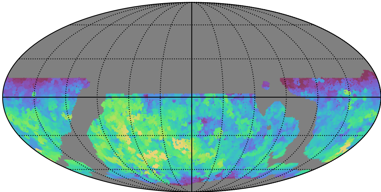
weather_cloudso10v3.4_10yrs WFD g band: Max fiveSigmaDepth
