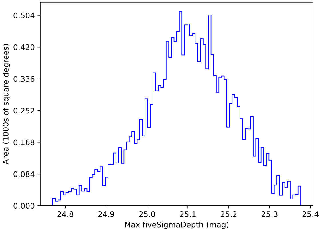
weather_cloudso10v3.4_10yrs WFD g band: Max fiveSigmaDepth
