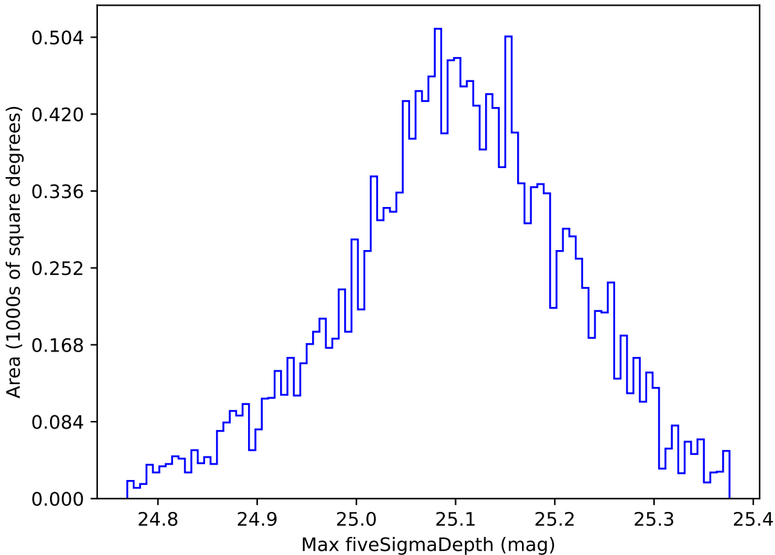
weather_cloudso10v3.4_10yrs WFD all bands: Max fiveSigmaDepth
