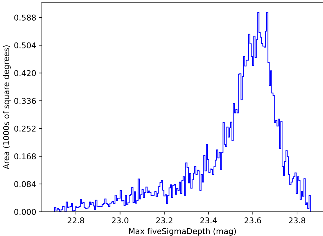
weather_cloudso10v3.4_10yrs All sky z band: Max fiveSigmaDepth
