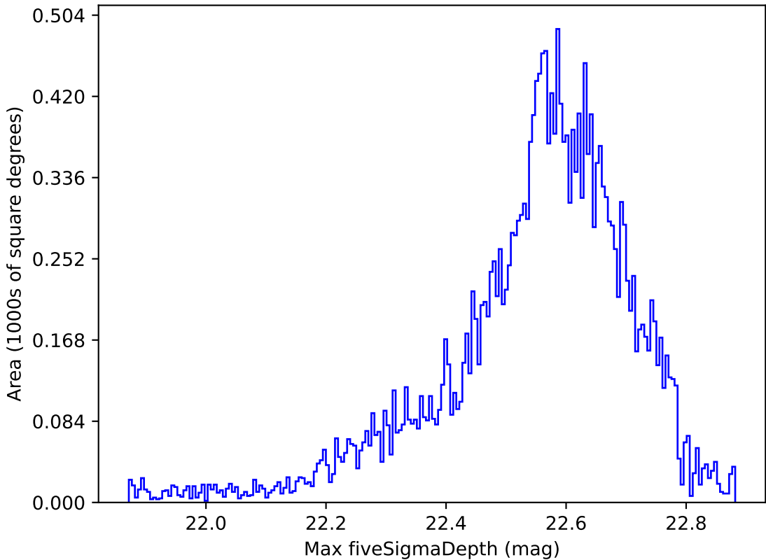
weather_cloudso10v3.4_10yrs All sky y band: Max fiveSigmaDepth
