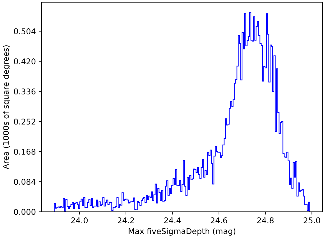
weather_cloudso10v3.4_10yrs All sky r band: Max fiveSigmaDepth
