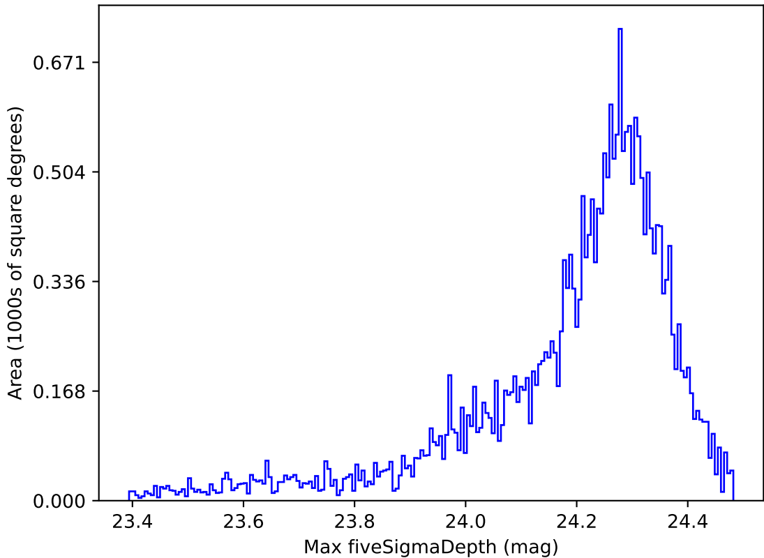
weather_cloudso10v3.4_10yrs All sky i band: Max fiveSigmaDepth
