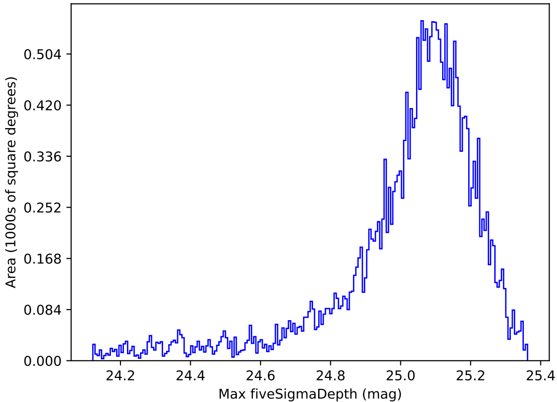
weather_cloudso10v3.4_10yrs All sky g band: Max fiveSigmaDepth
