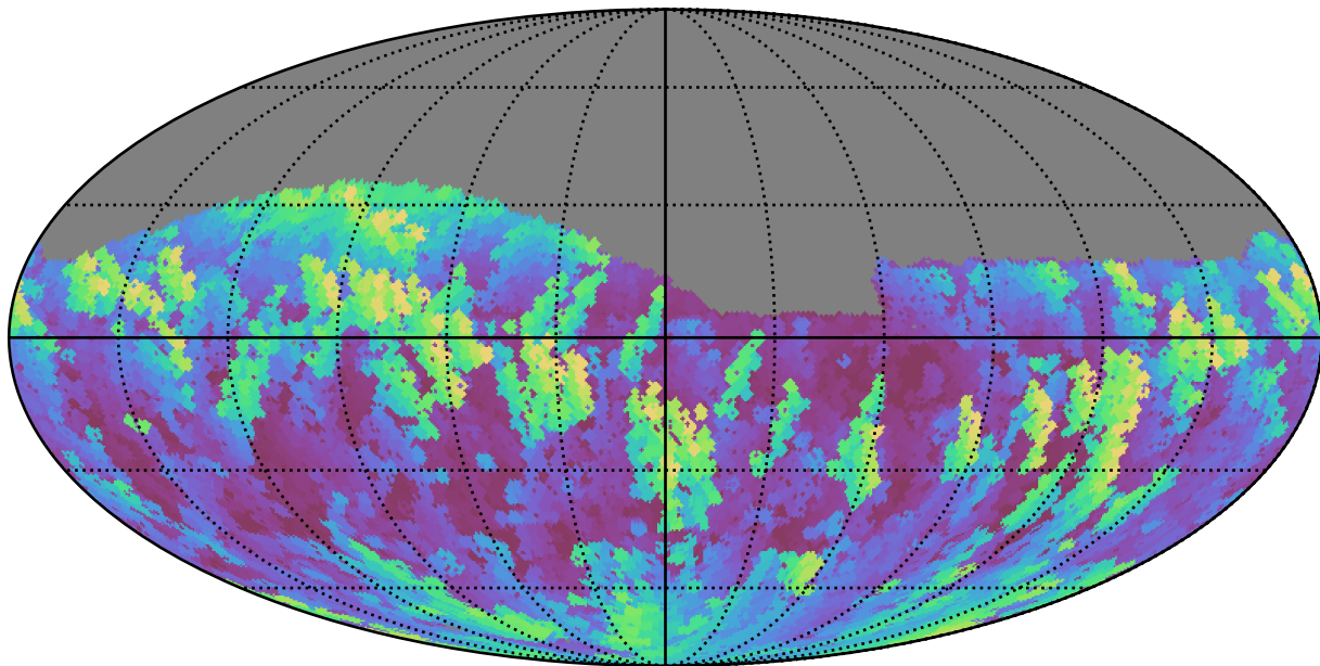
weather_cloudso10v3.4_10yrs Yr 1 z band: Max airmass
