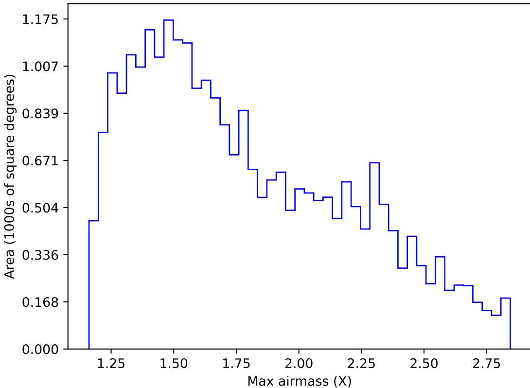
weather_cloudso10v3.4_10yrs Yr 1 z band: Max airmass
