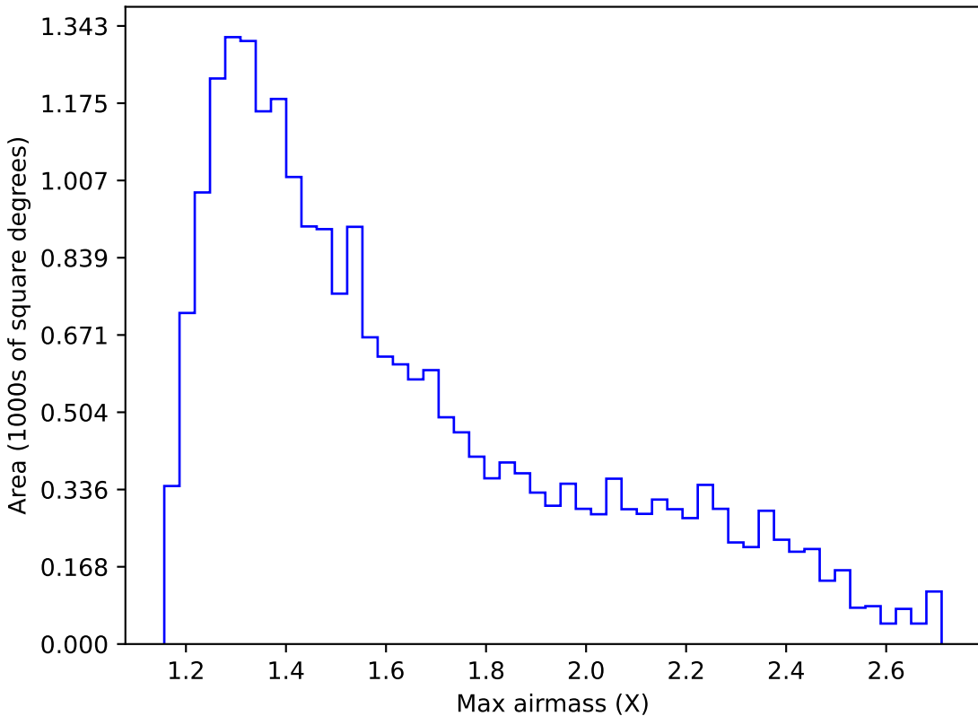
weather_cloudso10v3.4_10yrs Yr 1 y band: Max airmass
