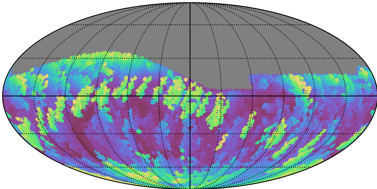
weather_cloudso10v3.4_10yrs Yr 1 r band: Max airmass
