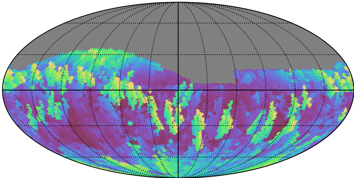
weather_cloudso10v3.4_10yrs Yr 1 i band: Max airmass
