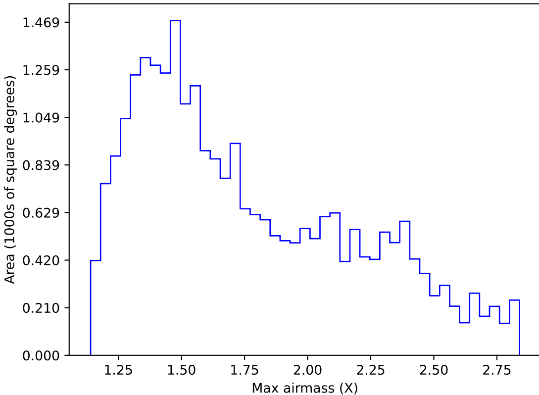
weather_cloudso10v3.4_10yrs Yr 1 i band: Max airmass
