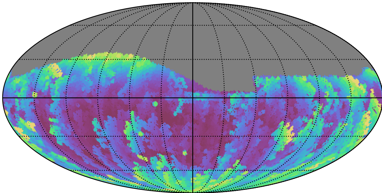
weather_cloudso10v3.4_10yrs Yr 1 g band: Max airmass
