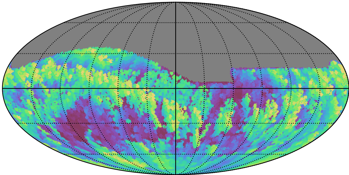
weather_cloudso10v3.4_10yrs Yr 1 all bands: Max airmass
