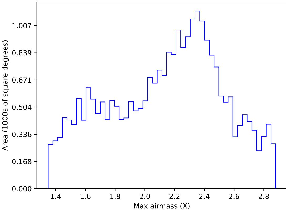
weather_cloudso10v3.4_10yrs Yr 1 all bands: Max airmass
