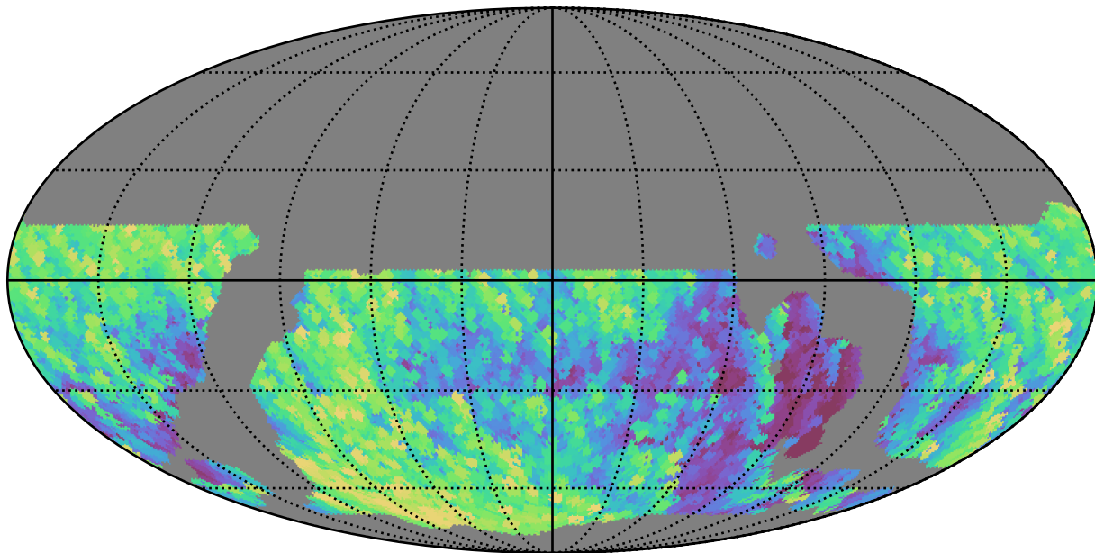
weather_cloudso10v3.4_10yrs WFD y band: Max airmass
