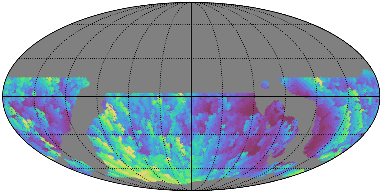
weather_cloudso10v3.4_10yrs WFD u band: Max airmass
