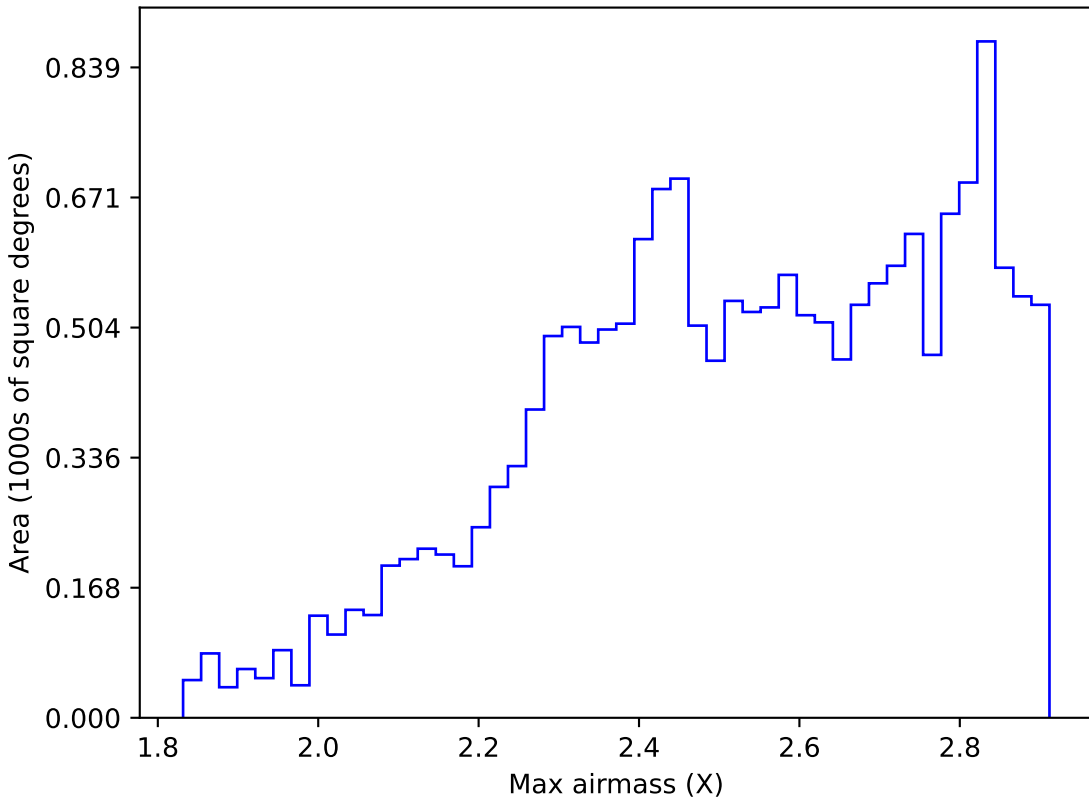
weather_cloudso10v3.4_10yrs WFD i band: Max airmass
