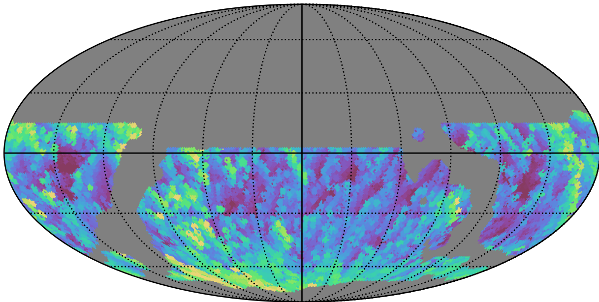
weather_cloudso10v3.4_10yrs WFD g band: Max airmass
