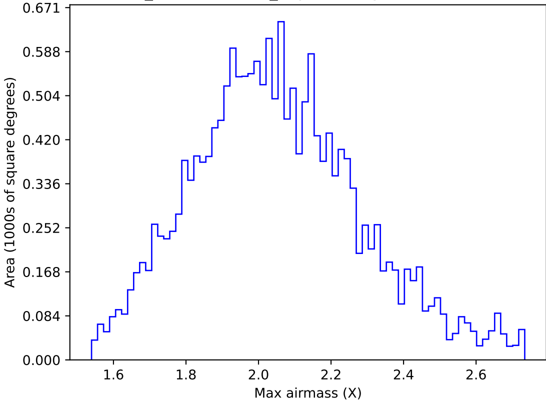
weather_cloudso10v3.4_10yrs WFD g band: Max airmass
