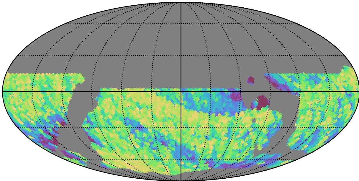
weather_cloudso10v3.4_10yrs WFD all bands: Max airmass
