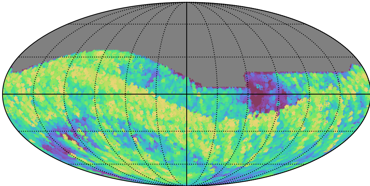
weather_cloudso10v3.4_10yrs All sky z band: Max airmass
