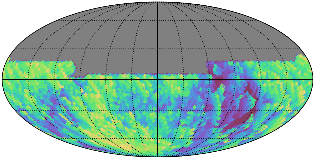
weather_cloudso10v3.4_10yrs All sky y band: Max airmass
