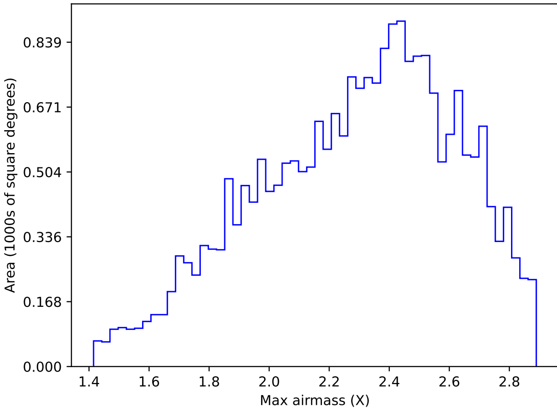
weather_cloudso10v3.4_10yrs All sky y band: Max airmass
