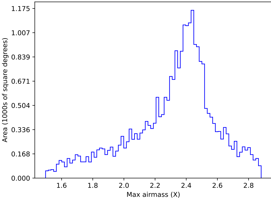
weather_cloudso10v3.4_10yrs All sky r band: Max airmass
