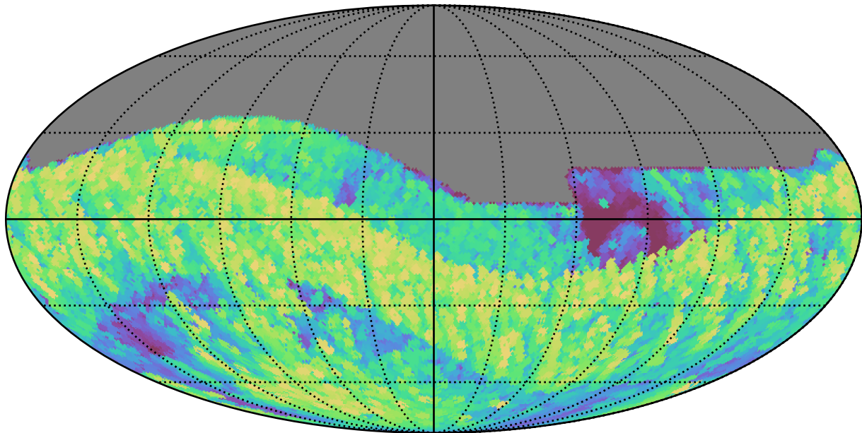
weather_cloudso10v3.4_10yrs All sky i band: Max airmass
