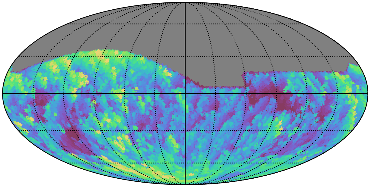
weather_cloudso10v3.4_10yrs All sky g band: Max airmass
