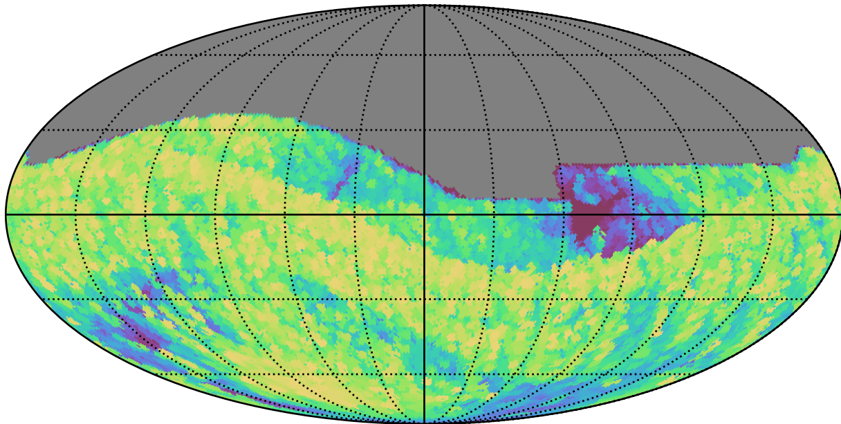
weather_cloudso10v3.4_10yrs All sky all bands: Max airmass
