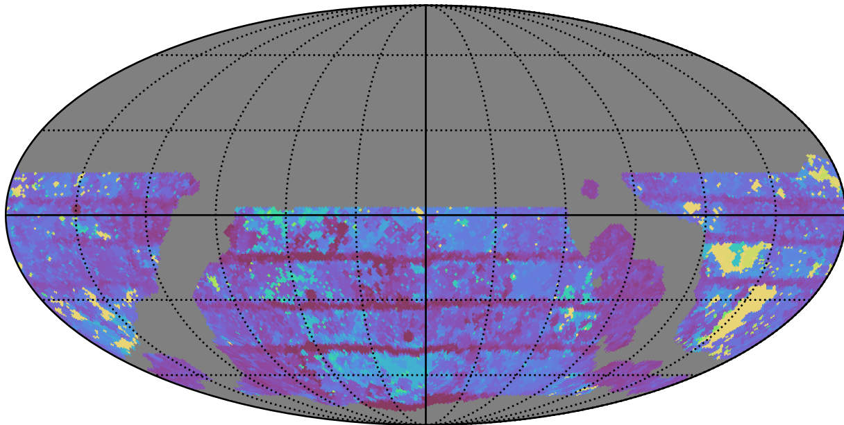
weather_cloudso10v3.4_10yrs WFD z band: Max Inter-Night Gap
