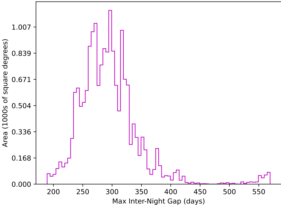
weather_cloudso10v3.4_10yrs WFD z band: Max Inter-Night Gap
