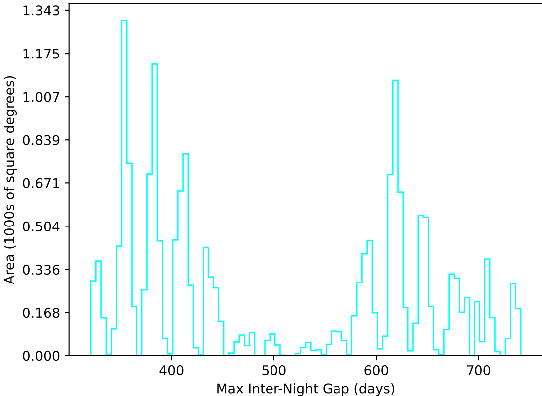
weather_cloudso10v3.4_10yrs WFD u band: Max Inter-Night Gap
