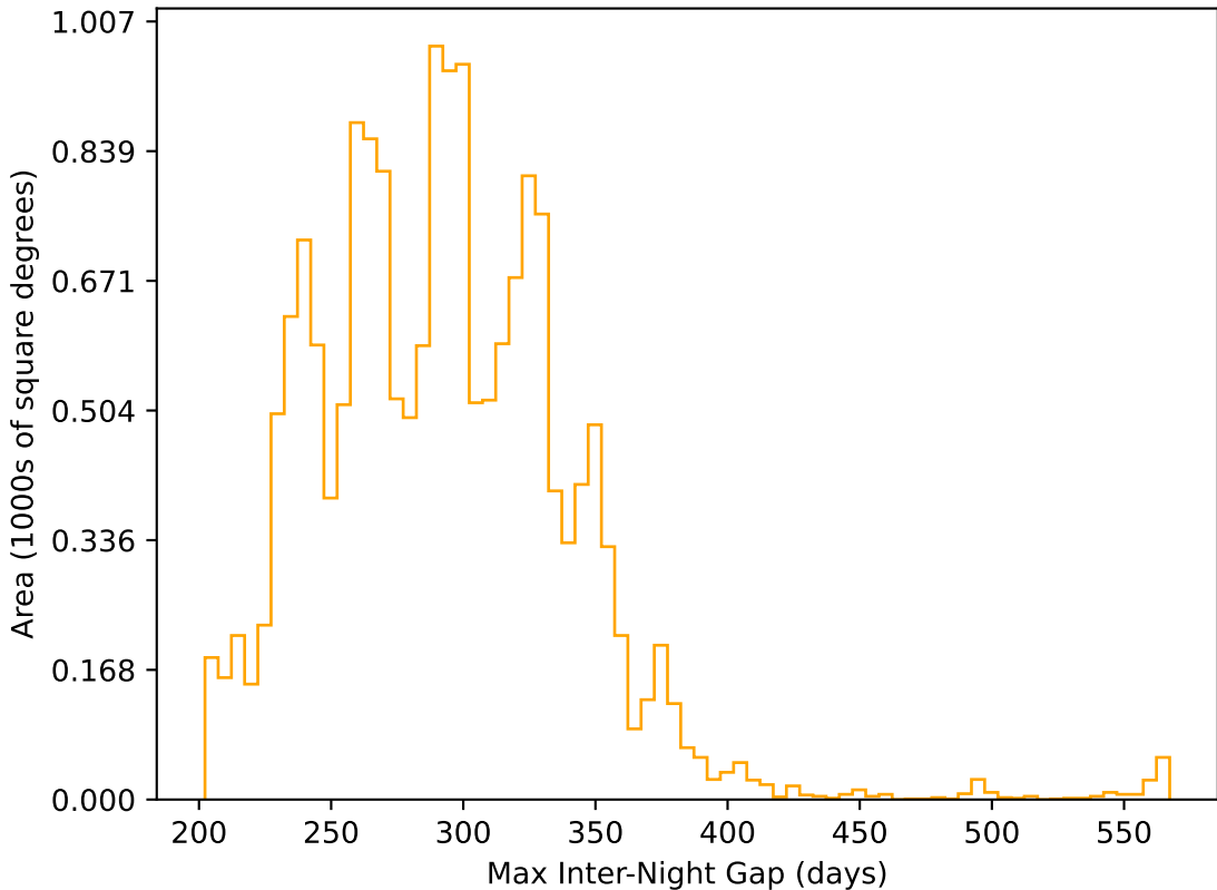
weather_cloudso10v3.4_10yrs WFD r band: Max Inter-Night Gap
