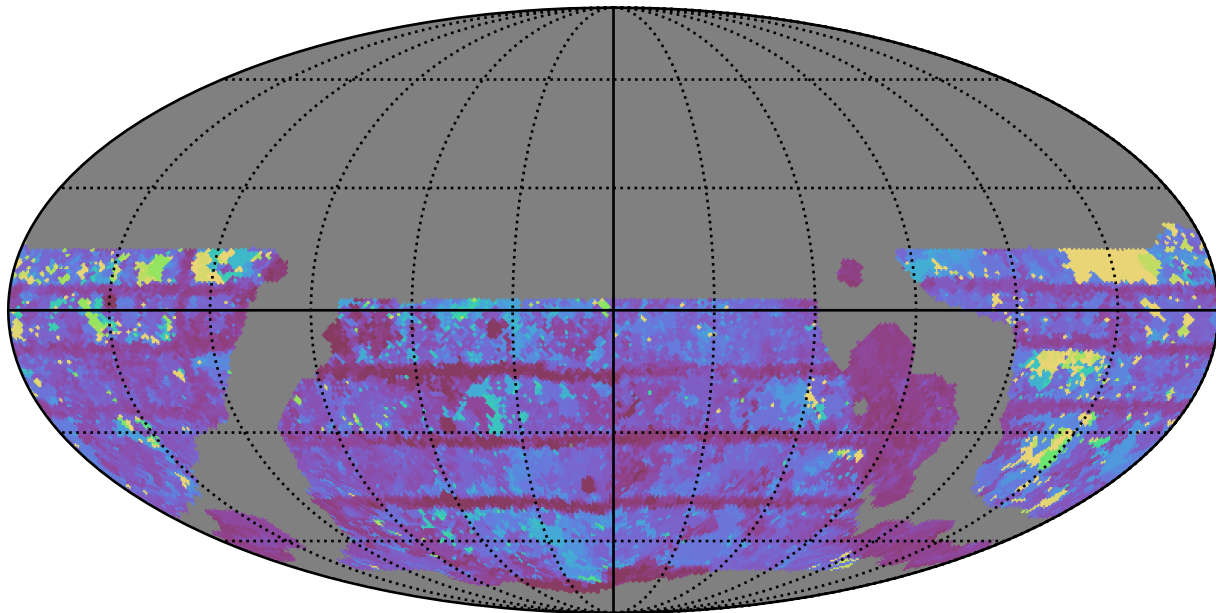
weather_cloudso10v3.4_10yrs WFD i band: Max Inter-Night Gap
