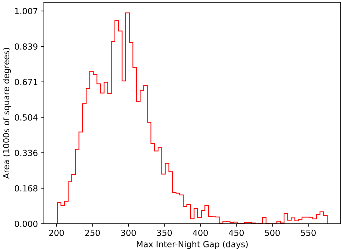
weather_cloudso10v3.4_10yrs WFD i band: Max Inter-Night Gap
