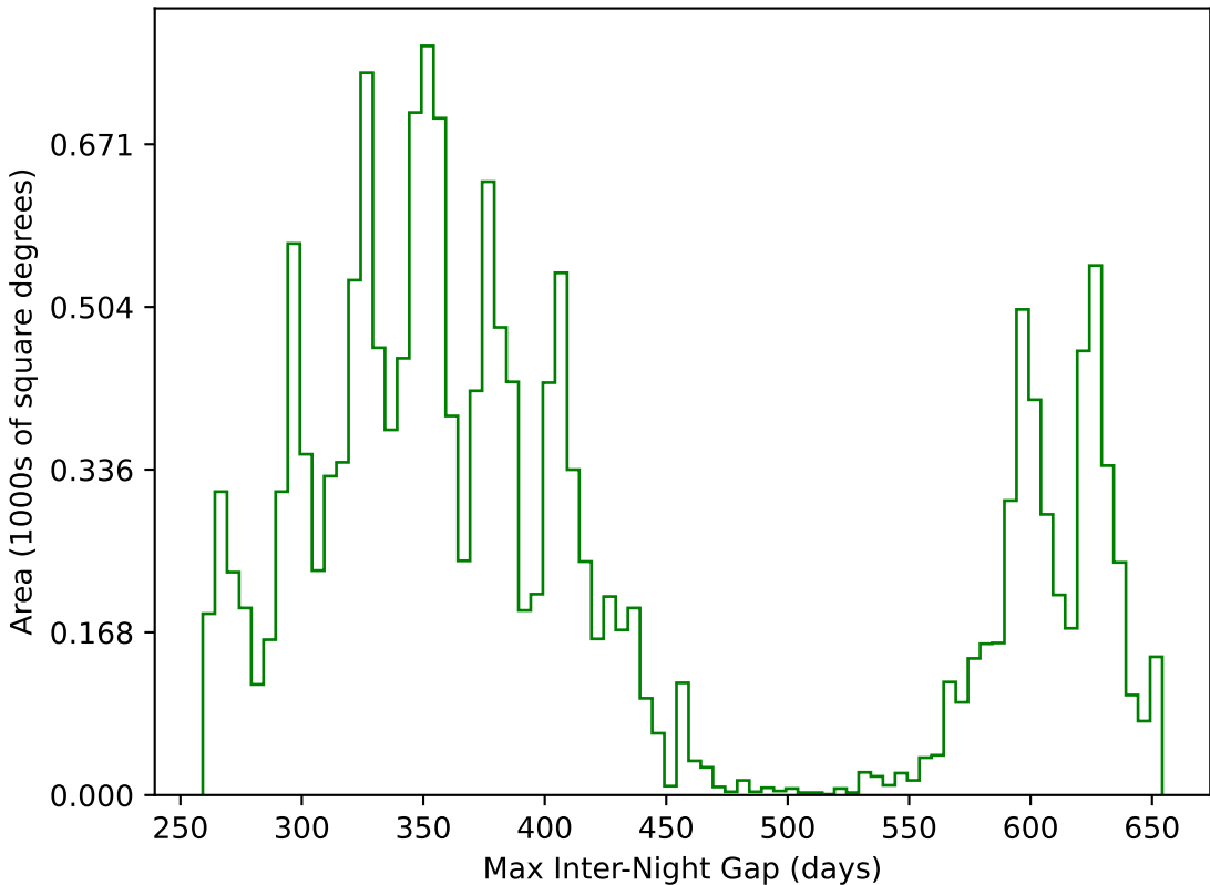
weather_cloudso10v3.4_10yrs WFD g band: Max Inter-Night Gap
