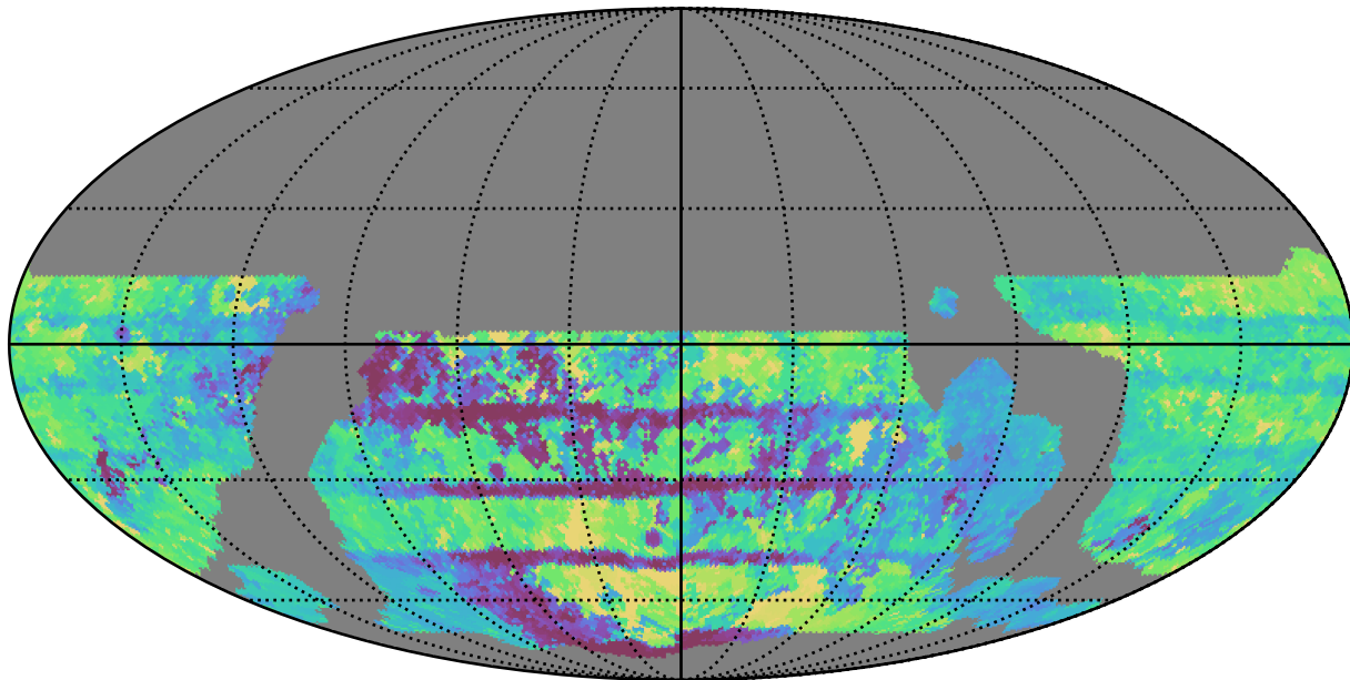
weather_cloudso10v3.4_10yrs WFD all bands: Max Inter-Night Gap
