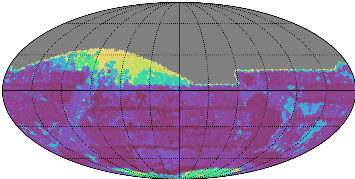
weather_cloudso10v3.4_10yrs All sky z band: Max Inter-Night Gap
