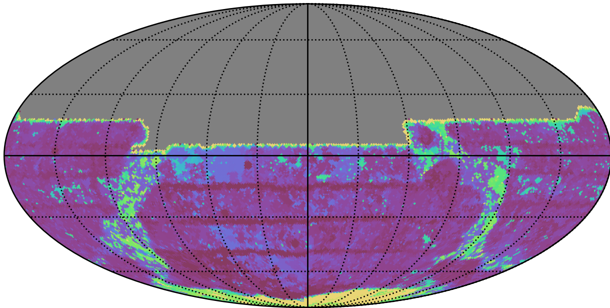
weather_cloudso10v3.4_10yrs All sky y band: Max Inter-Night Gap
