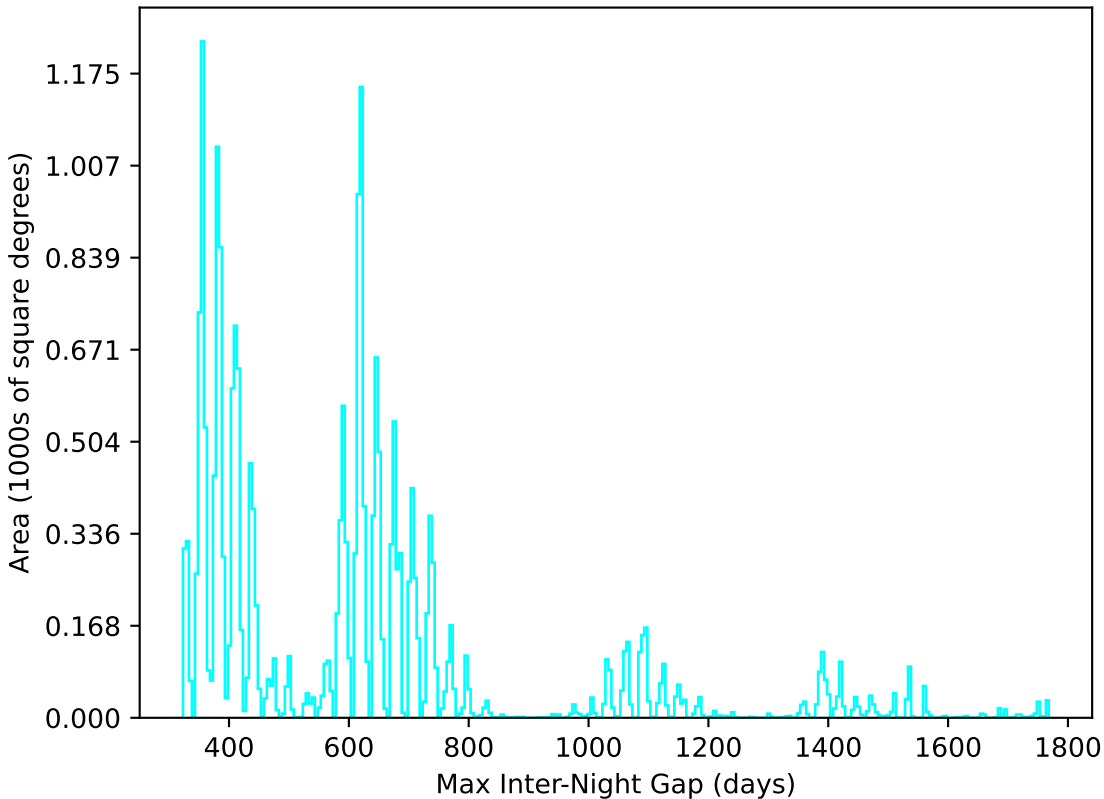
weather_cloudso10v3.4_10yrs All sky u band: Max Inter-Night Gap
