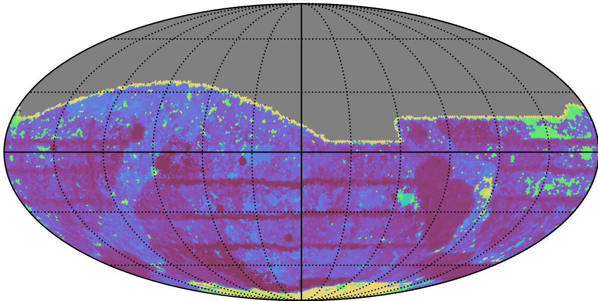
weather_cloudso10v3.4_10yrs All sky r band: Max Inter-Night Gap
