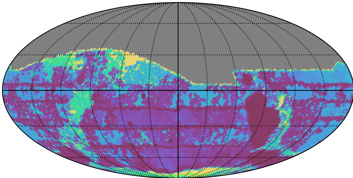
weather_cloudso10v3.4_10yrs All sky g band: Max Inter-Night Gap
