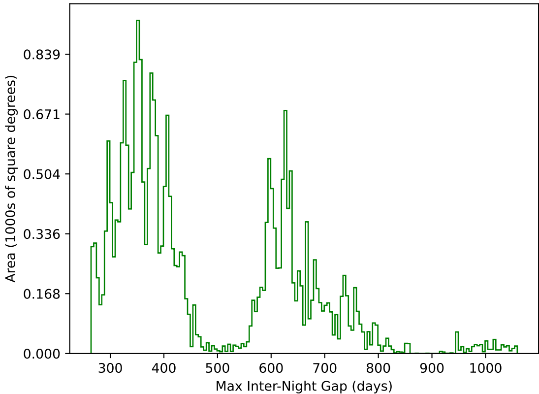
weather_cloudso10v3.4_10yrs All sky g band: Max Inter-Night Gap
