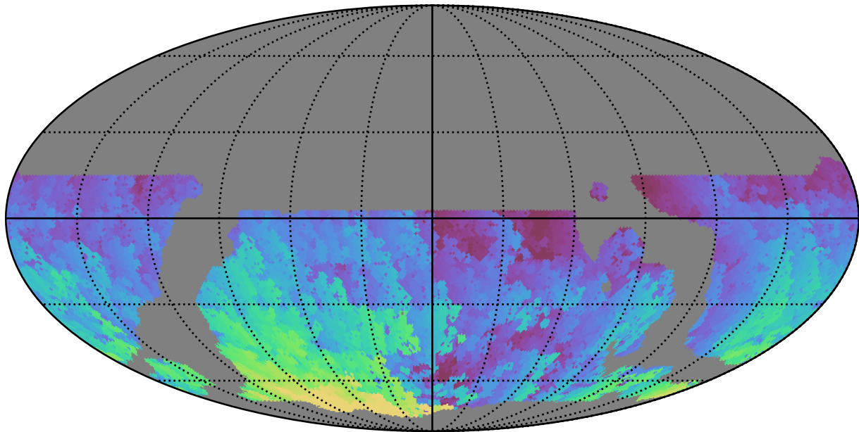
weather_cloudso10v3.4_10yrs WFD u band: Max HA
